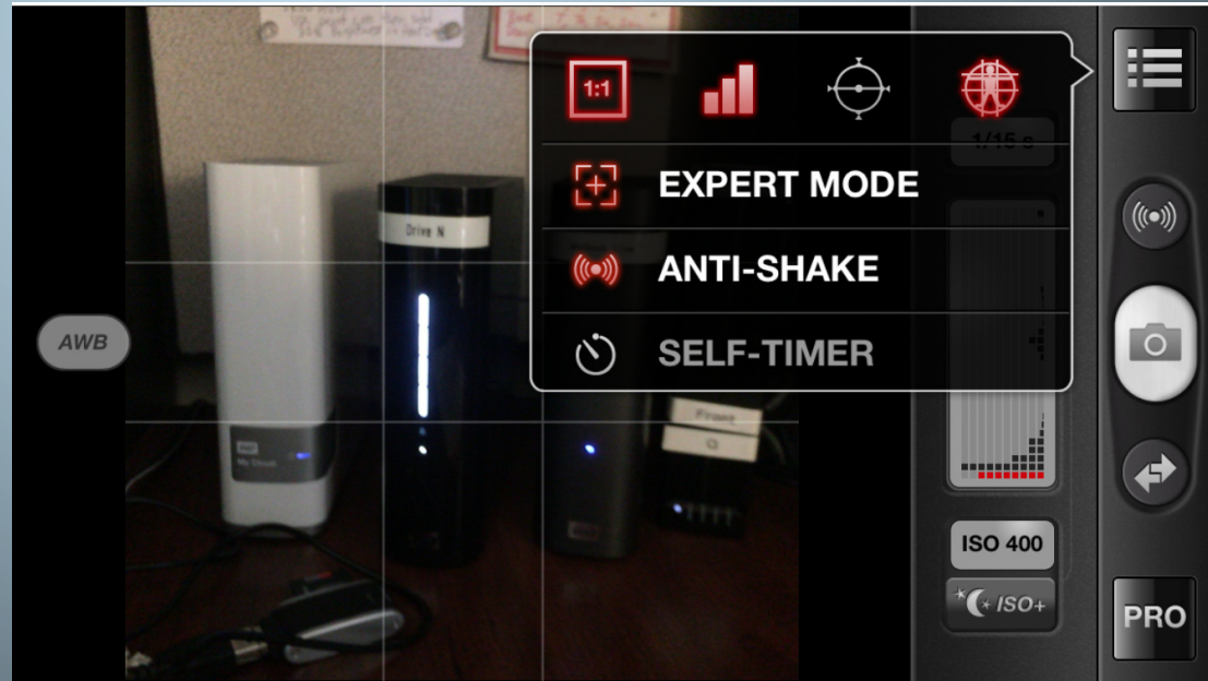
Camera Pro
